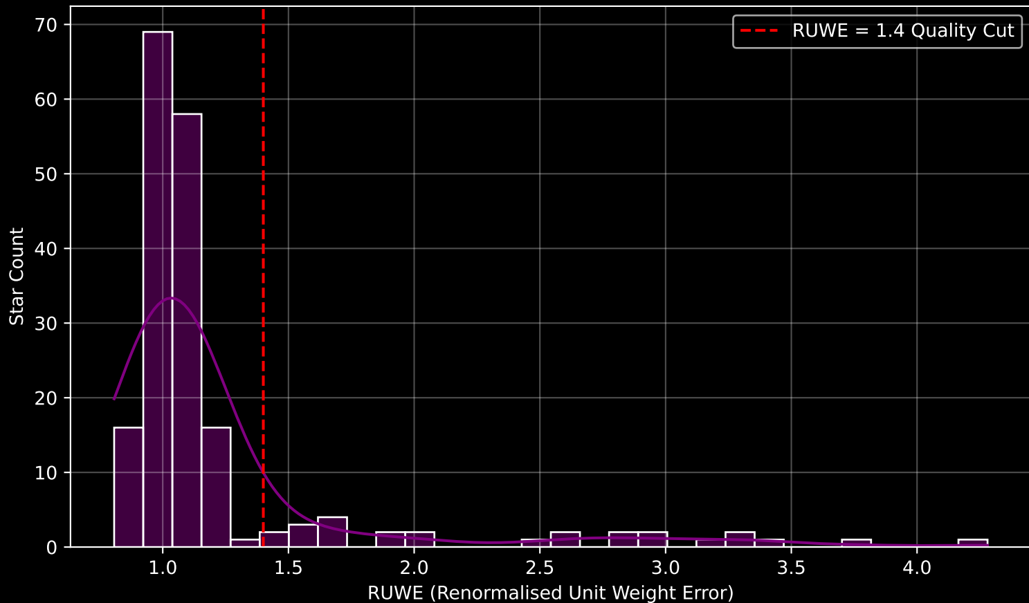
GAPOGEE DR17 Field [260+60] RUWE Distribution (n= 186)
