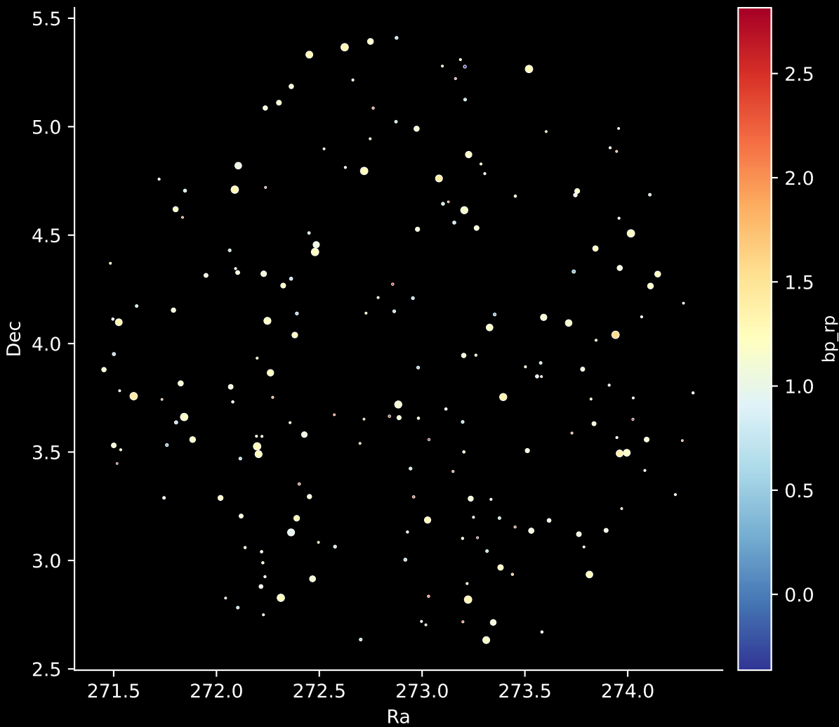
APOGEE DR17 Field: [260+60] Stars: 196
