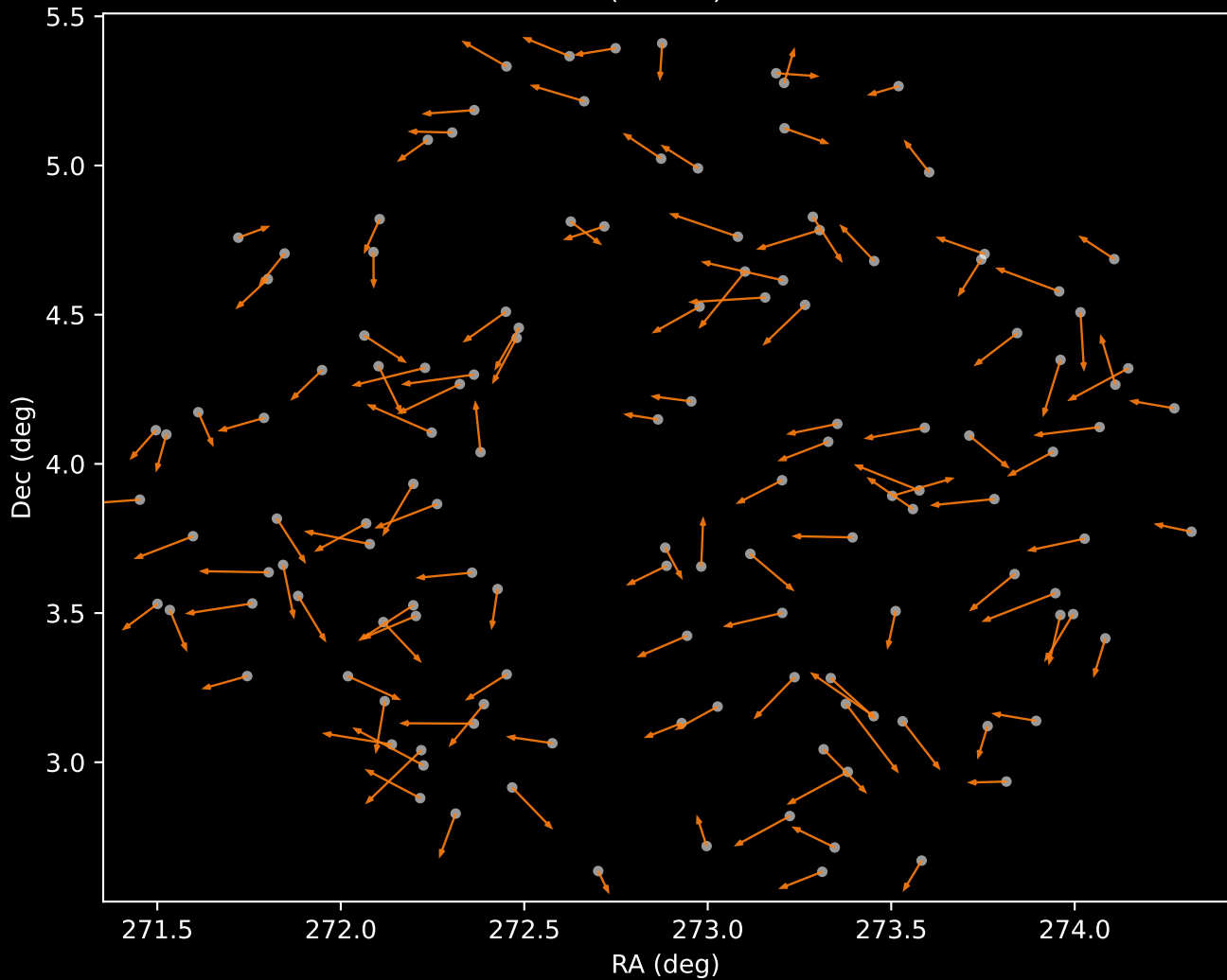
APOGEE DR17 Cluster 2 Proper Motion Vectors (n=133)
