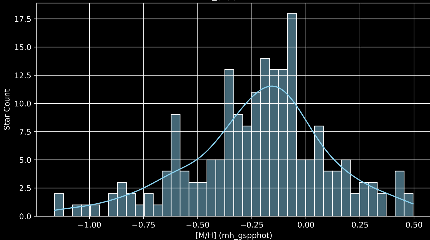
APOGEE DR17 Field: [260+60 [M/H] (mh_gspphot) (n= 195)
