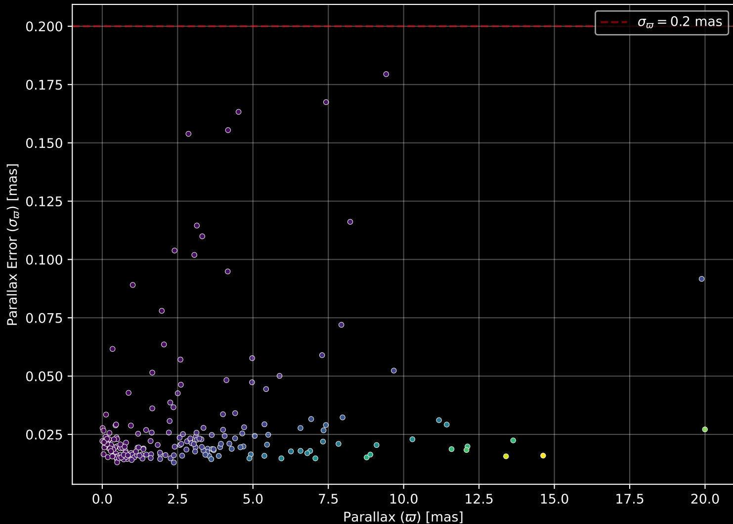
APOGEE DR17 Field: [260+60] Parallax Quality (n= 196)
