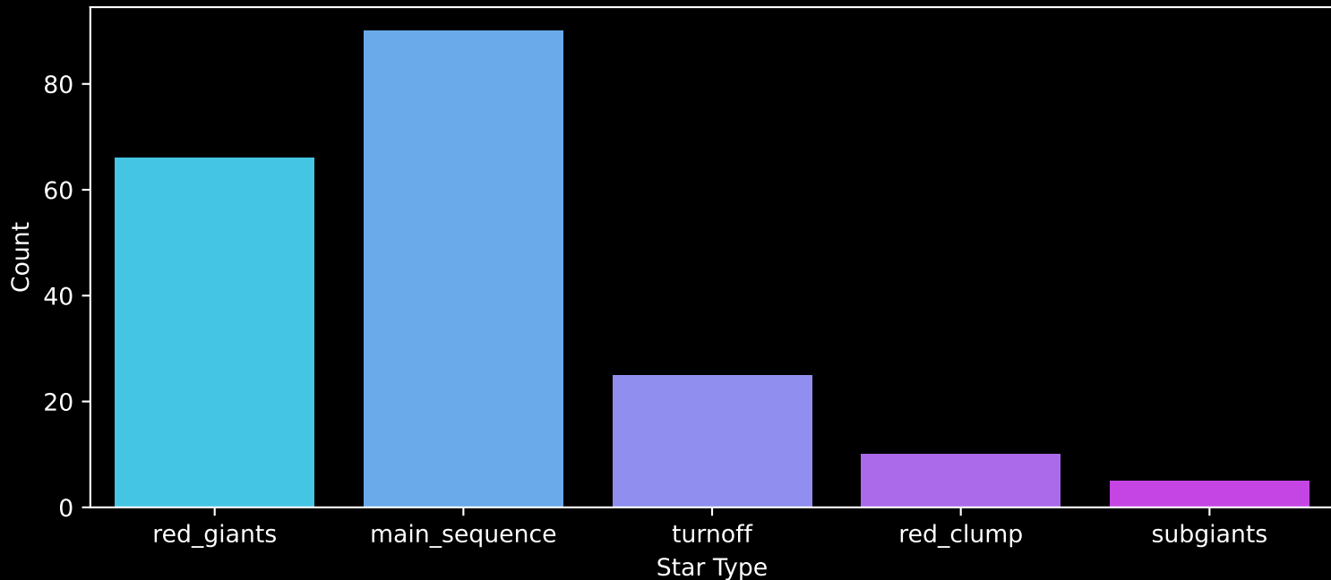
APOGEE DR17 Field: [260+60] Count plot of Star Type
