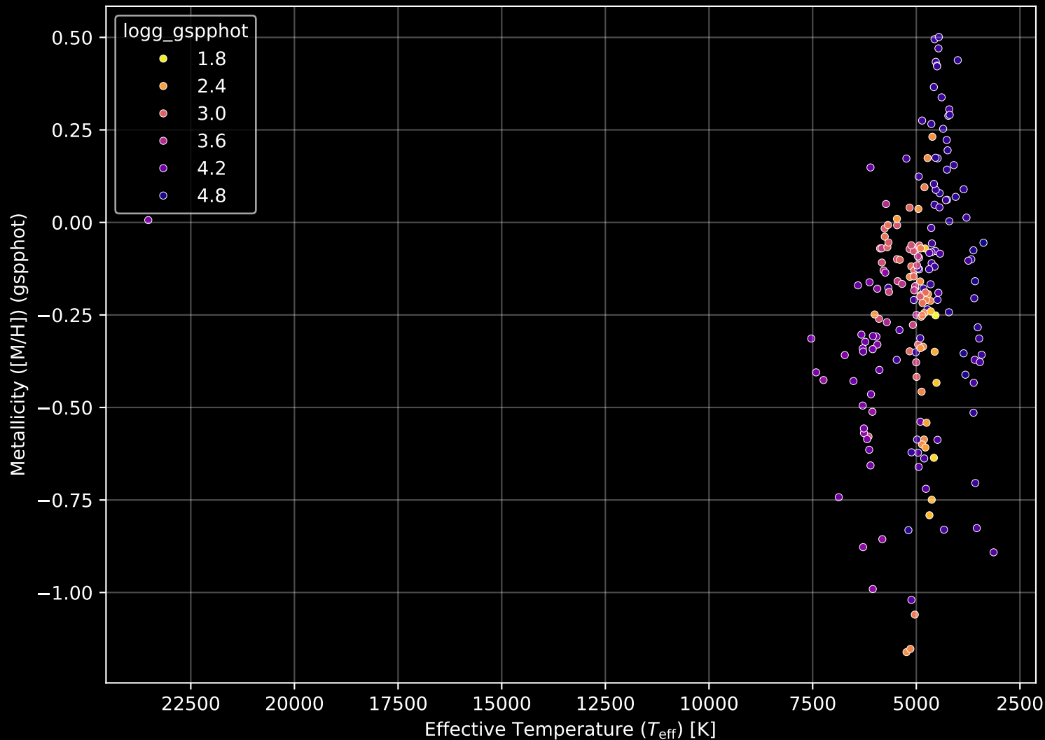
APOGEE DR17 Field: [260+60] Stellar Population Parameters (n= 196)
