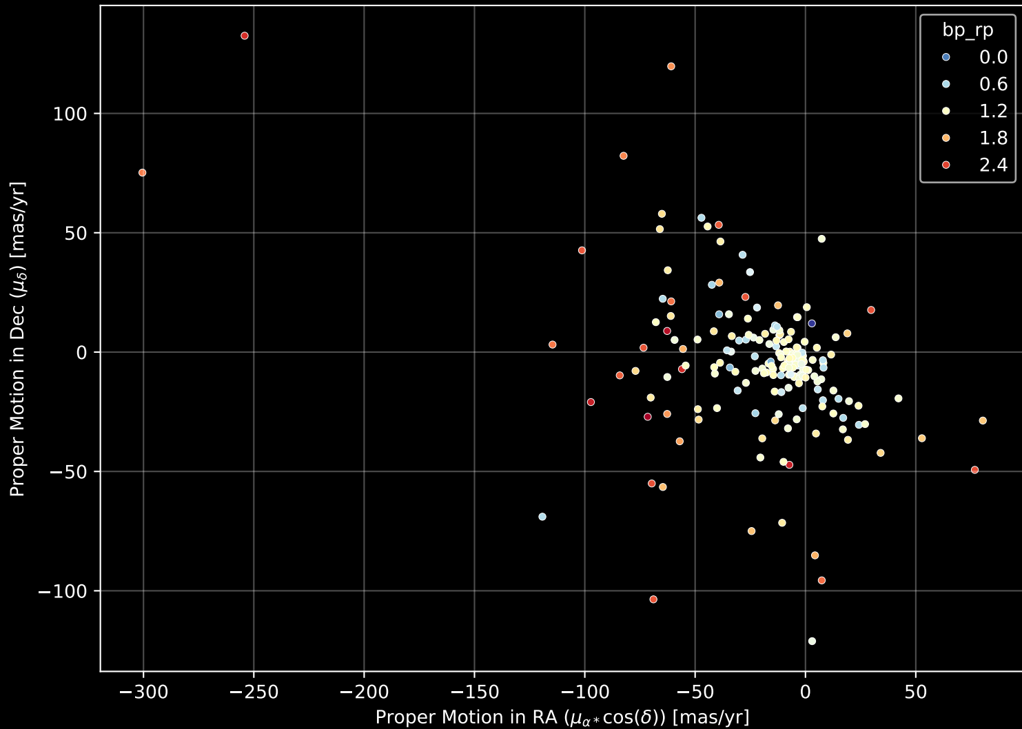
APOGEE DR17 Field: [260+60] Proper Motion Diagram (n= 196)
